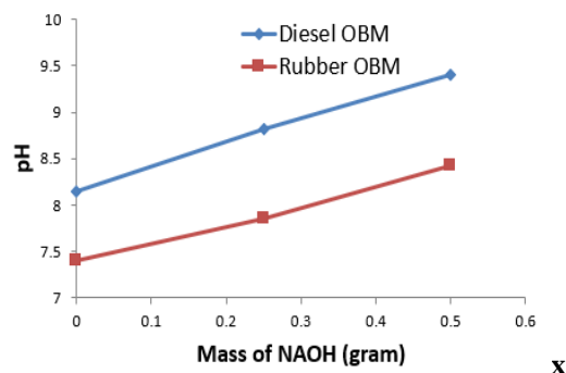
Figure 14. Comparison of mud pH with addition of NAOH
