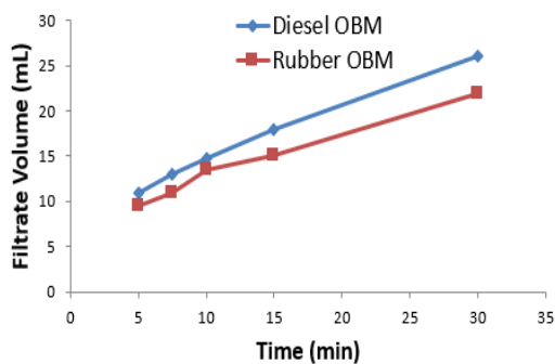
Figure 13. Time comparison of filtrate loss
