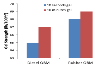
Figure 8. Diesel and rubber OBMs gel strength
