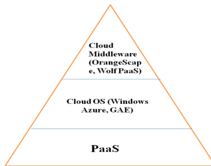
Figure 5. PaaS layers
