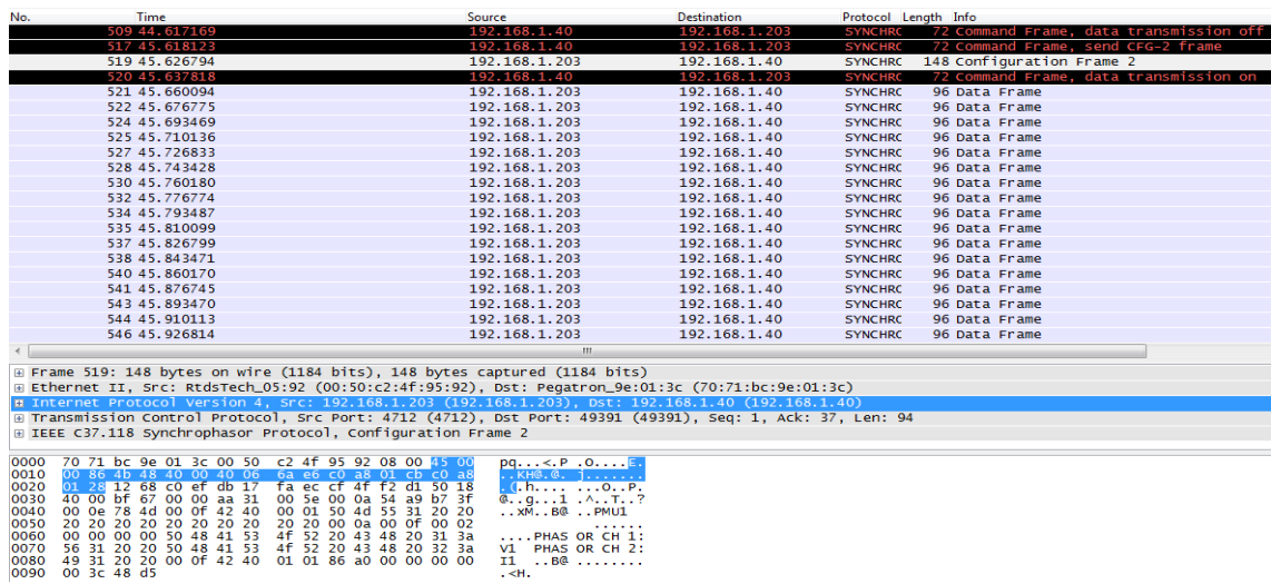
Figure 6. Synchrophasor Messages for PMU-2 and PDC-2 Captured Using A Network Protocol Analyzer-Wireshark
