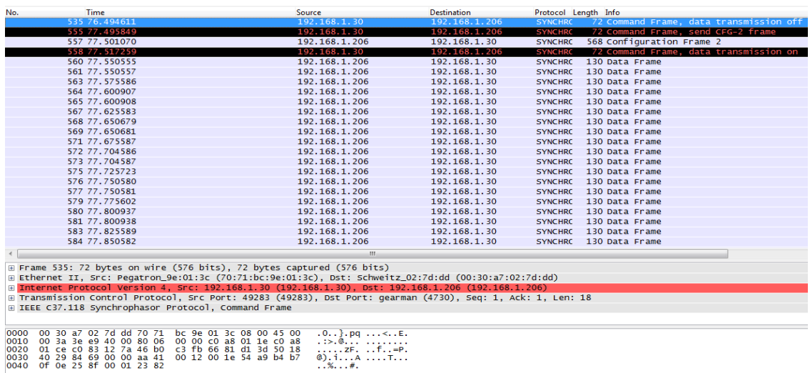
Figure 7. Synchrophasor Messages for PMU-3 and PDC-3 Captured Using A Network Protocol Analyzer-Wireshark
