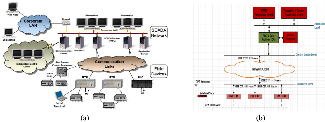
Figure 1. Wide Area Measurement Architecture Using (a) SCADA-Based Measurements; (b) Synchrophasor-Based Measurement
