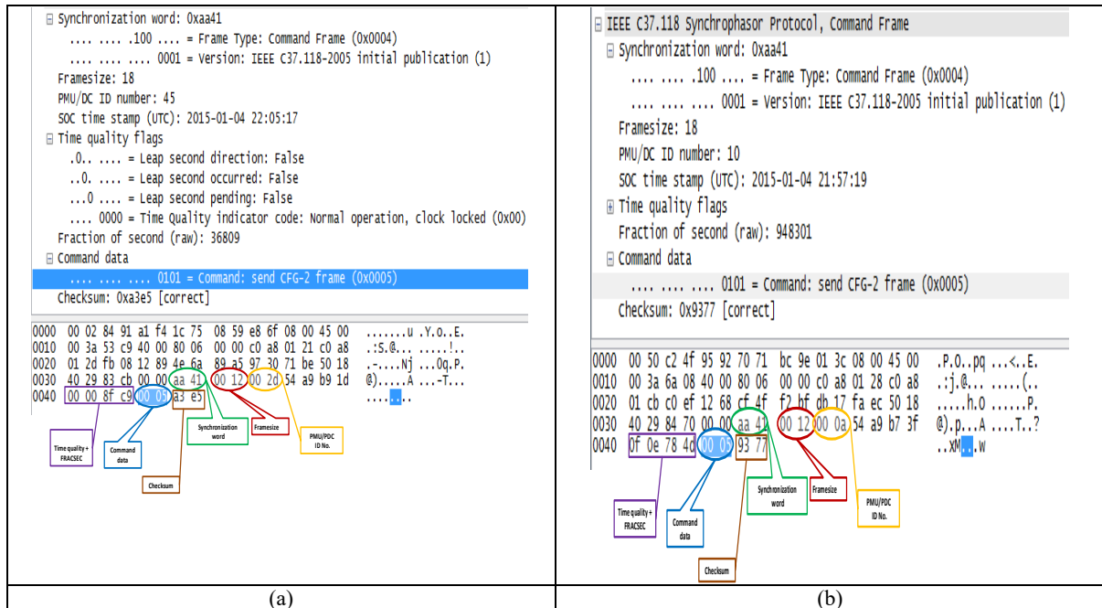
Figure 8. Wireshark Capture of Command Fram from (a) PDC-1 to PMU-1; (b) PDC-2 to PMU-2
