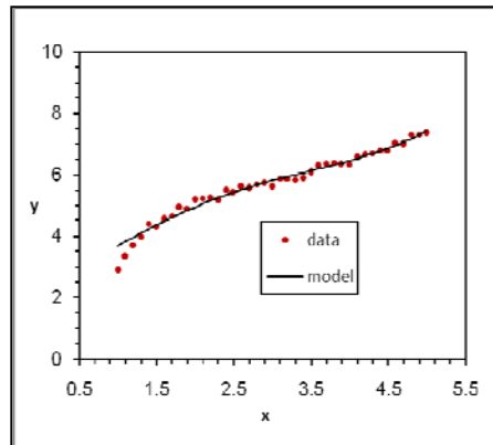
Figure 5. Cubic spline curve for n=2
