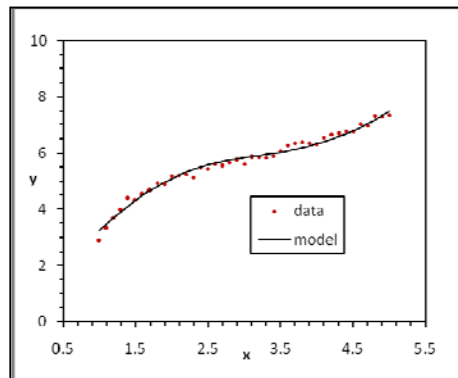
Figure 6. Cubic spline curve for n=3
