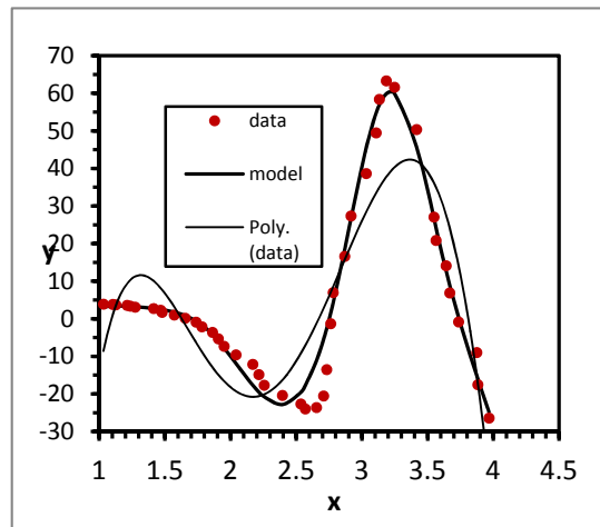
Figure 9. Piecewise cubic spline method for n=7
