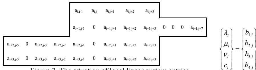
Figure 3. The situation of local linear system entries.
