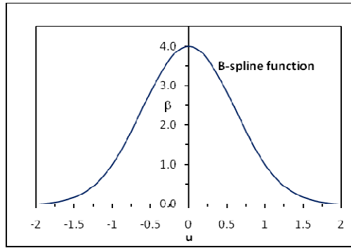
Figure 1. B-spline function
