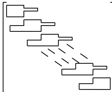
Figure 4. The situations of local system entries.
